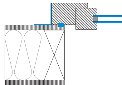
> Alternative with joint sealing tape or round cord
